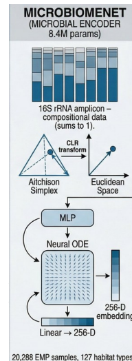
20,288 EMP samples, 127 habitat types. rRNA amplicon data (compositional, sums to 1) is mapped from the Aitchison simplex to Euclidean space via CLR transform, processed by an MLP and Neural ODE to produce a 256-D embedding.
